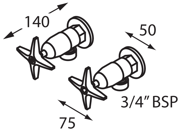
APP-C064 3/4N3S Washing Machine Cocks
