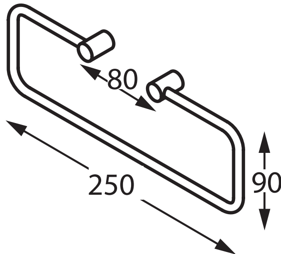
VIV-C031 Towel Ring
